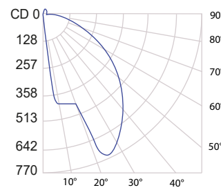
Accent light 3000K,90CRI -1350
