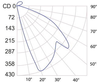
Accent light 3000K,90CRI - 240
